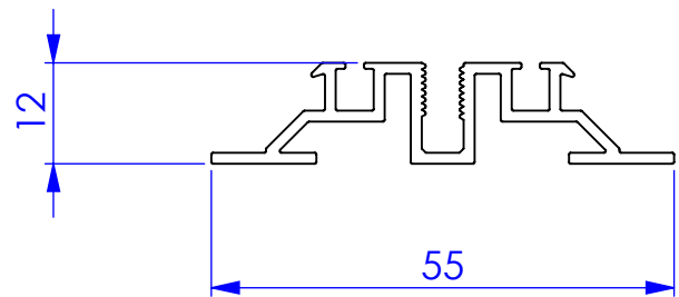
DETAIL A SCALE 1 : 1
