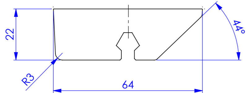
DETAIL A SCALE 1 : 1
